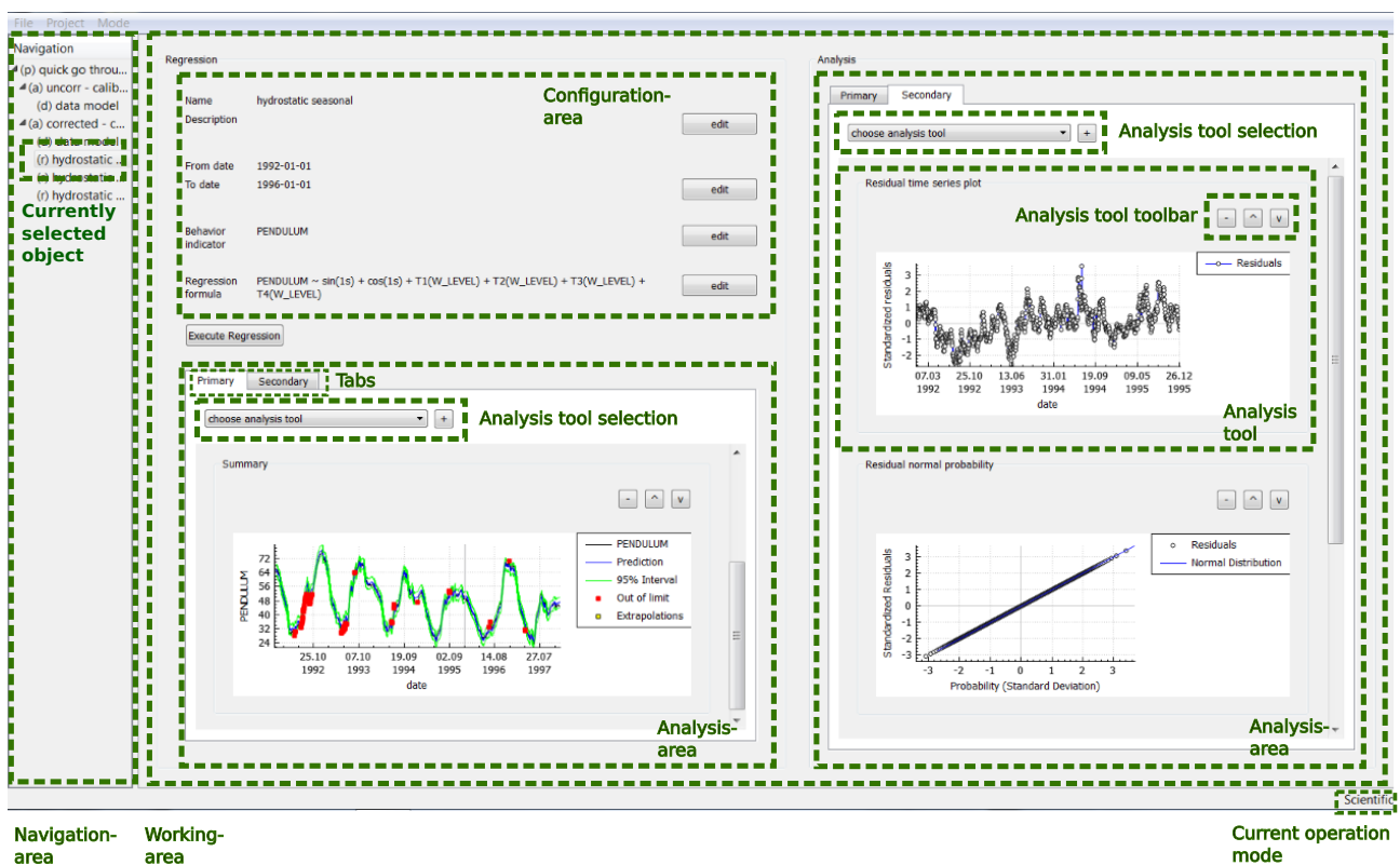
Fig. 1.3 User interface concept
