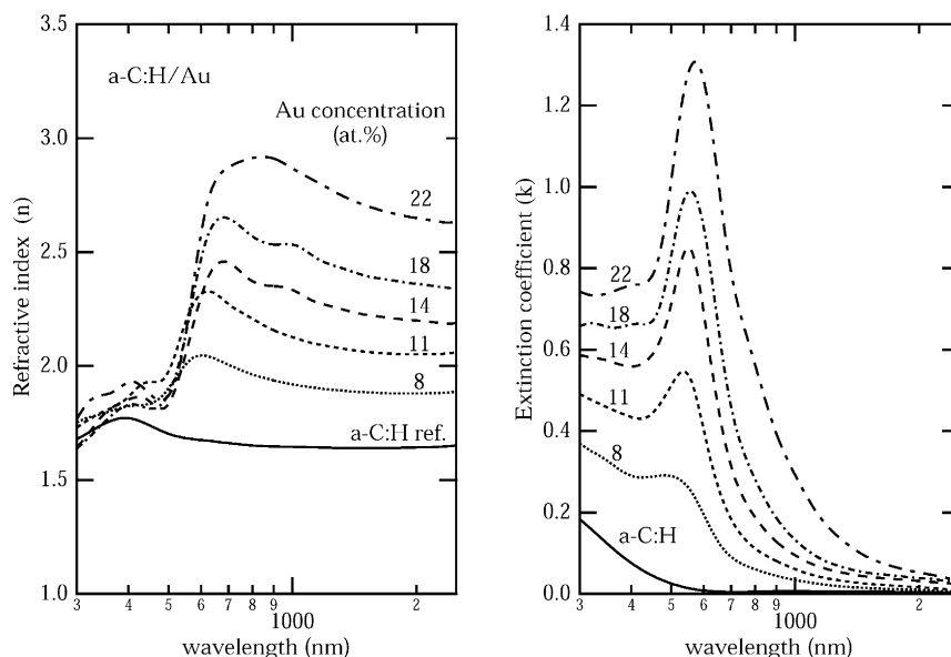
Fig. 5. Refractive index n and extinction coefficient k of a-C:H/Au films with different Au concentrations (given here in at%) along with an a-C:H reference film (Gampp, 1996).
