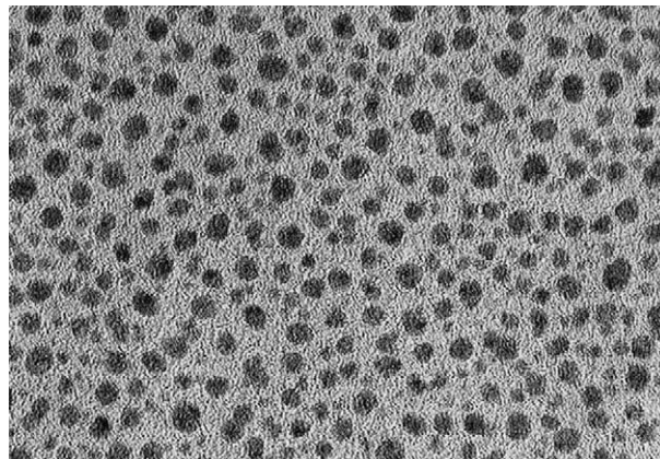
Fig. 4. TEM image of an a-C:H/Au nanocomposite film. The Au particles appear as dark aggregates. The Au content of the film is 11.9 at%. The mean cluster diameter is about 2 nm (Gampp, 1996).
