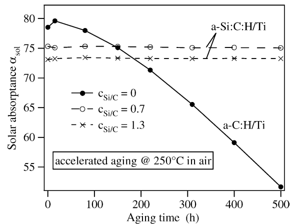
Fig. 8. Accelerated aging test of single layered solar absorber coatings at 250 °C in air. Displayed is the evolution of the solar absorptance \alpha_{sol} for two series of coatings on aluminum substrates (with and without Ti precoating). The solar absorptance \alpha_{sol} of the a-C:H/Ti coatings drops down significantly, while \alpha_{sol} of the a-Si:C:H/Ti coatings remains constant (Schüller et al., 2001).
