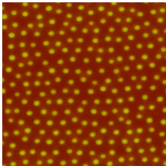
Fig. 2. Atomic force microscopy (AFM) image of 8 nm Au clusters prepared by the micellar method (image size 1 \times 1 \mu\text{m} , z-range 20 nm) (Boyen et al., 2002).
