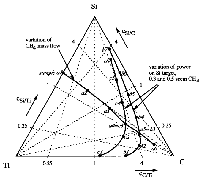
Fig. 7. Compositions of a-Si 1-x C x :H/Ti films, visualized in the concentration triangle Ti–C–Si. The solid lines indicate the dependence of the film composition on the process parameters CH 4 mass flow and power on the Si target. The labels a1,...,c6 denote different samples used in the experiment (Schüller and Oelhafen, 2001).
