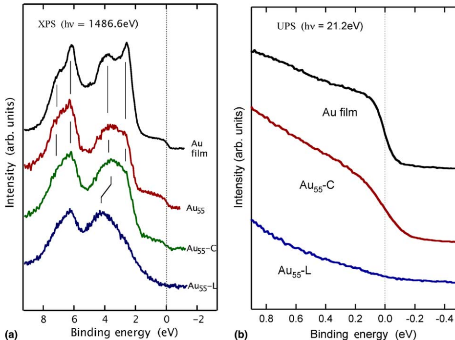
Fig. 1. (a) XPS valence band spectra of a Au reference film, naked supported Au clusters with a diameter of 1.6 nm, a monomolecular layer of the intact cluster compound ( \text{Au}_{55}\text{-L} ) and the compound after prolonged X-ray irradiation causing the Cl desorption ( \text{Au}_{55}\text{-C} ). (b) UPS valence band spectra showing the vicinity of the Fermi energy. Note the absence of the Fermi edge in the \text{Au}_{55}\text{-L} sample (Boyen et al., 2001).
