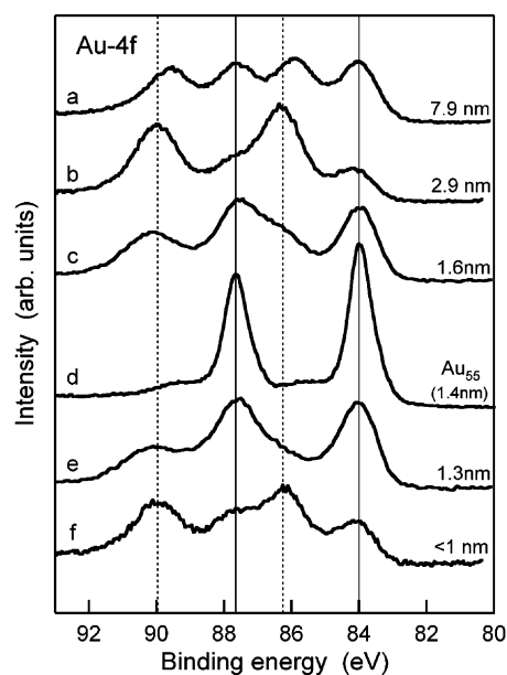
Fig. 3. Au 4f core level spectra of Au particles (size 1–8 nm) obtained after exposure to reactive oxygen species provided by an in situ rf-plasma. The vertical lines indicate the binding energy positions corresponding to elemental Au (Boyen et al., 2002).
