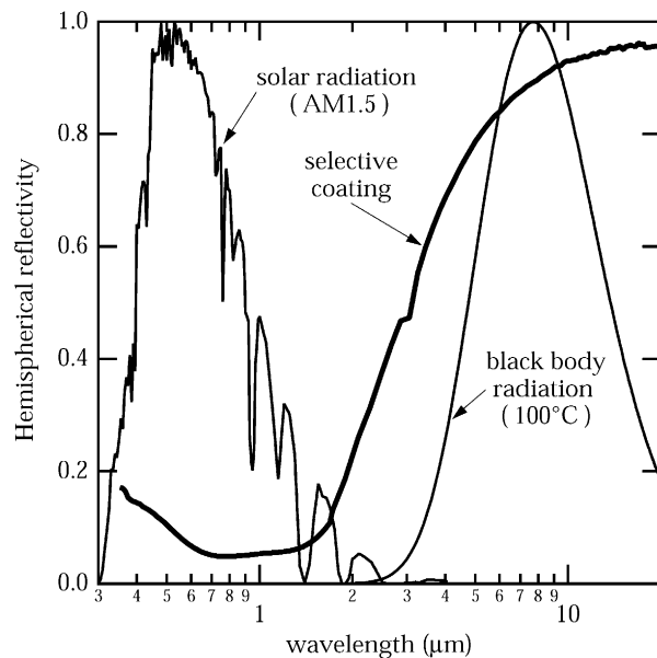
Fig. 6. Solar radiation AM1.5, black body radiation at 100^\circ\text{C} and hemispherical reflection of an optically selective a-C:H/Cr coating (Gampp, 1996).
