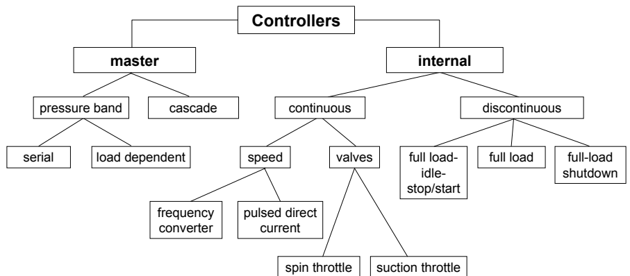
Fig. 1: Control of compressed air systems
